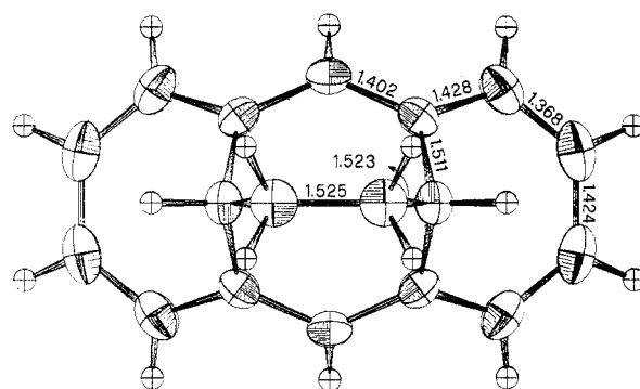
Figure 4. Bond lengths in 1,6:8,13-butane-1,4-diylidene[14]annulene.
